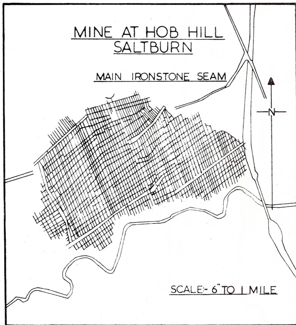
Typical ironstone mining plan after partial extraction stage.
